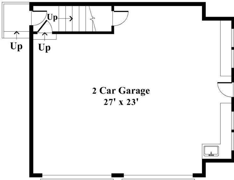
First Level - Garage
