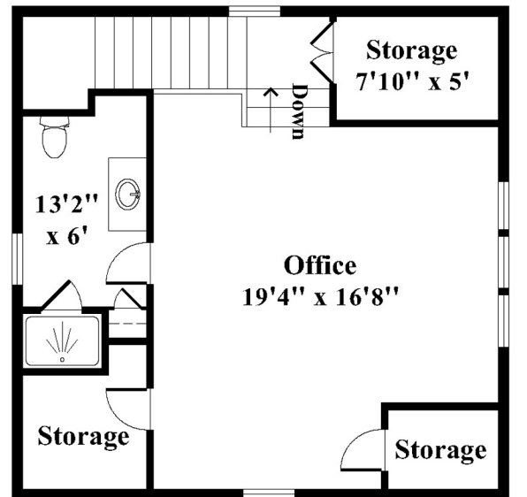
Second Level - Garage
